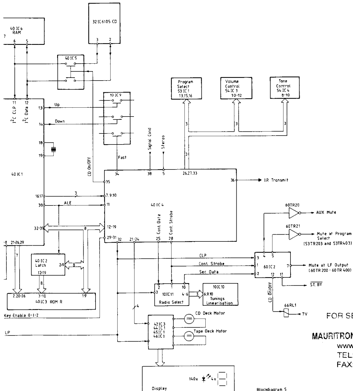
Blockdiagram 5
