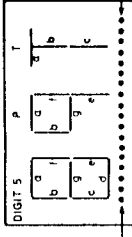
2DP2 PIN ASSIGNMENT (BOTTOM VIEW)
